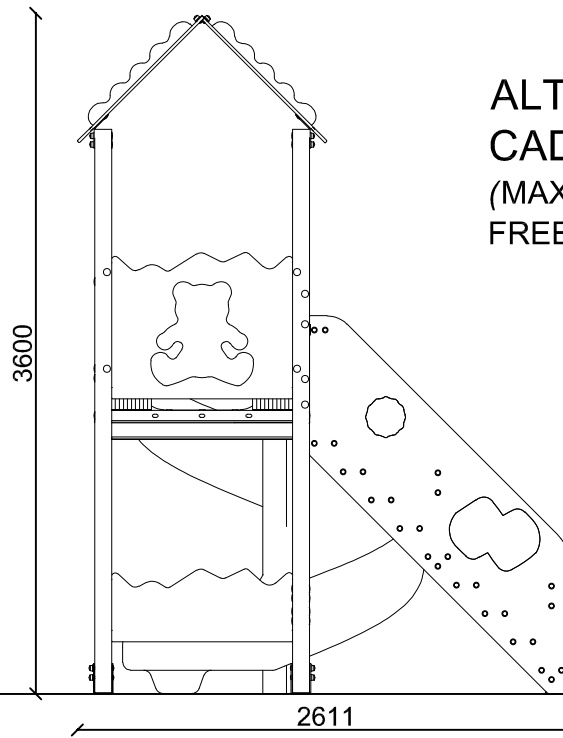
VISTA LATERALE (LATERAL VIEW)
